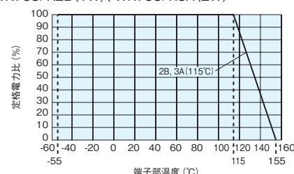
端子部温度 WK73S/R2B(1W)、WK73S/R3A(2W)
