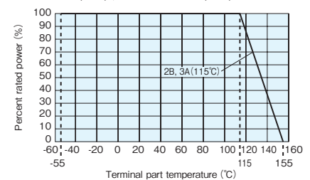
Terminal part temperature WK73S/R2B(1W)、WK73S/R3A(2W)
