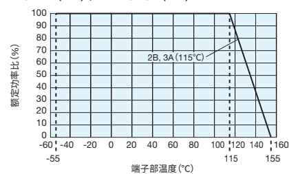
端子部温度 WK73R2B (1W)、WK73R3A (2W)
